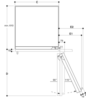
Wall clearance RB 472/RC/RF/RW
